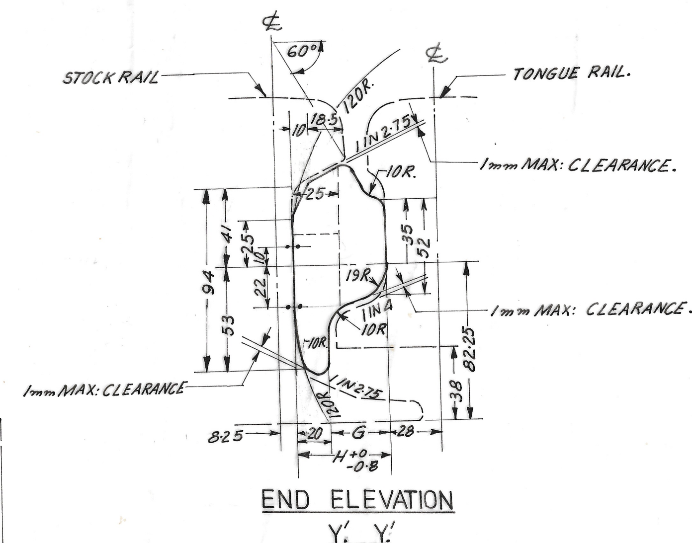
END ELEVATION Y. Y.
